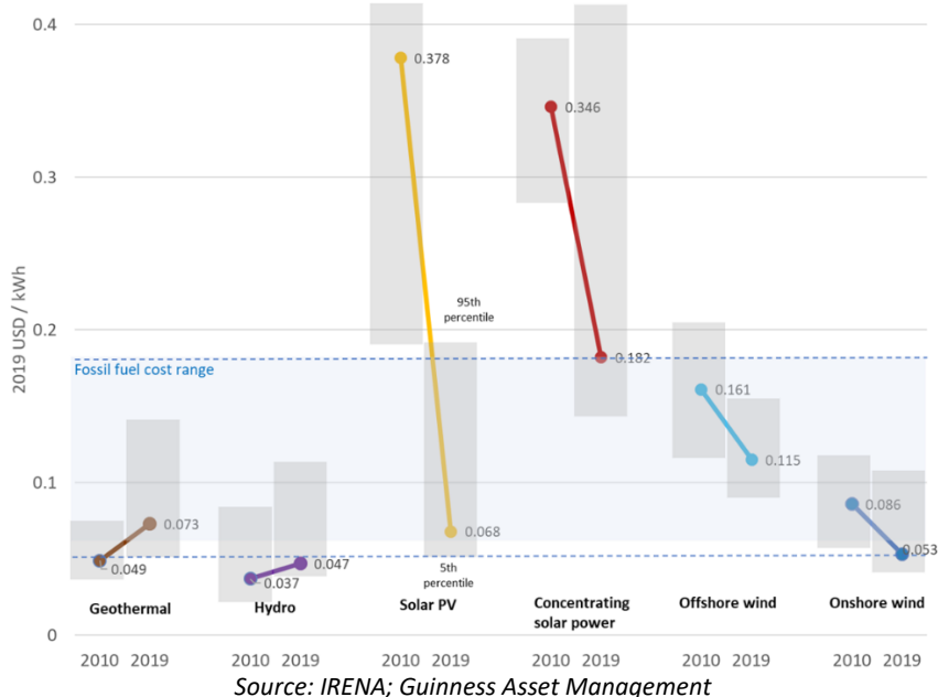
Global LCOE of utility-scale renewable power generation technologies (2010–2019)
